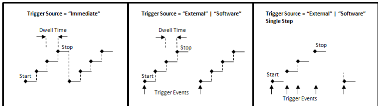
Figure 72. Frequency StepTiming
